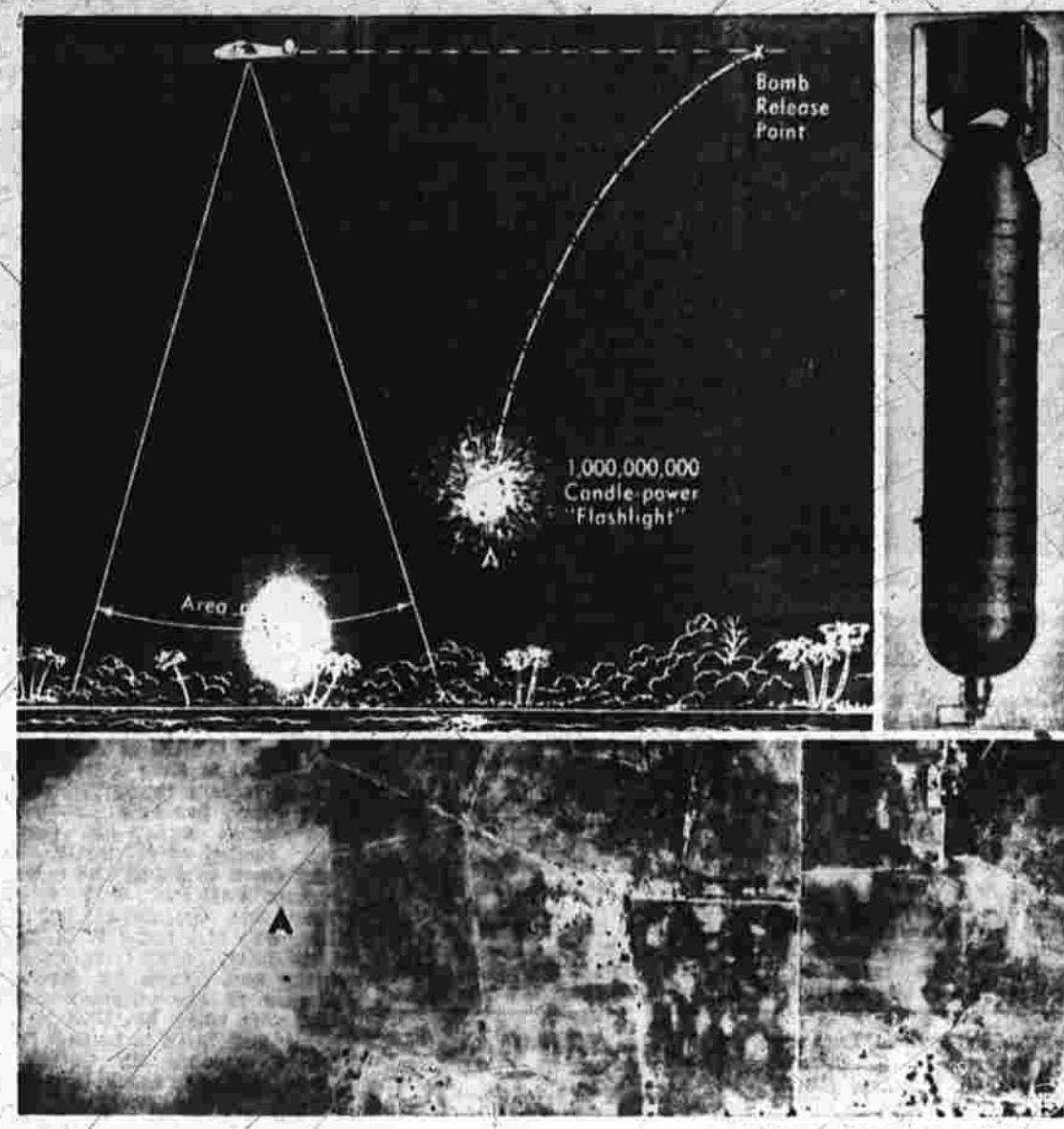
Diagram and photos above show how Army aerial reconnaissance photographers of night missions now "bomb" their photobombs with a super-duper "night-buster" flashlight beam, pictured at top, right. Weighing 92 pounds, it contains 25 pounds of flashlight powder, provides about a billion candlepower flash. It is used to explode at a point behind the plane, as shown in diagram. Explosion lights up target area and also activates photo-target area and also activates photo-target area and also activates photo-target area.
